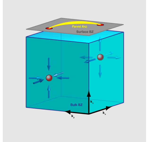
FIG. 1: Schematic image of the structure of the Weyl semimetal in momentum space. Two diaboli- cal points are shown in red, within the bulk three-dimensional Brillouin zone. The excitations near each diaboli- cal point behave like Weyl fermions. Each point is a source or sink of the flux (i.e., a monopole in momentum space) of the U(1) Berry connec- tion, defined from the Bloch wave functions, as indicated by the blue arrows. The grey plane indicates the surface Brillouin zone, which is a projection of the bulk one. Wan et al. show that an odd number of surface Fermi arcs termi- nate at the projection of each diaboli- cal point, as drawn here in yellow. In the iridium pyrochlores studied in the paper, a nonschematic picture would be significantly more complex, as there are 24 diaboli- cal points rather than 2. (Credit: Alan Stonebraker)
