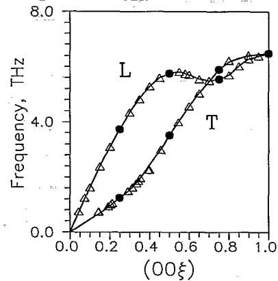
FIG. 1. Calculated phonon dispersions in Nb (full lines) along the (001) direction in the Brillouin zone using the linear-response method described in the paper. Results of total-energy supercell calculations (circles) using the full-potential LMTO method [15] as well as experiment [17] (triangles). L, longitudinal; T, transverse modes.
