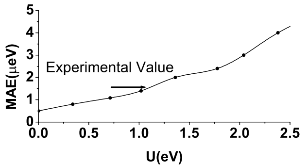
Fig. 2. The magneto-crystalline anisotropy energy \text{MAE} = E(111) - E(001) for Fe as function of U . The experimental MAE is marked by arrow ( 1.4 \mu\text{eV} ). The values of exchange parameter J for every value of U are chosen to hold the magnetic moment of 2.2 \mu_B .
