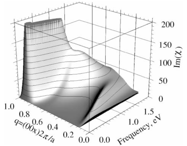
Fig. 7. Calculated \text{Im}[\chi_{\pm}(\mathbf{q}, \omega)] ( \text{Ry}^{-1} ) for Cr.
