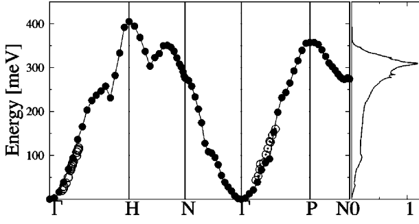
Fig. 4. Comparison between calculated using frozen magnon method and experimental [38] spin wave spectrum for Fe.
