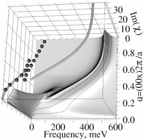
Fig. 6. Calculated \text{Im}[\chi_{\pm}(\mathbf{q}, \omega)] (arb.units) for Ni. Experimental data [65] are indicated by balls.
