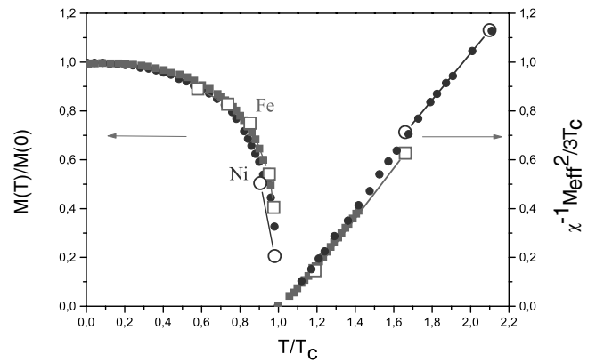
Fig. 8. Temperature dependence of ordered moment and the inverse ferromagnetic susceptibility for Fe (open square) and Ni (open circle) compared with experimental results for Fe (square) and Ni (circle) (from Ref. 97). The calculated moments were normalized to the LDA ground state magnetization (2.2 \mu_B for Fe and 0.6 \mu_B for Ni).
