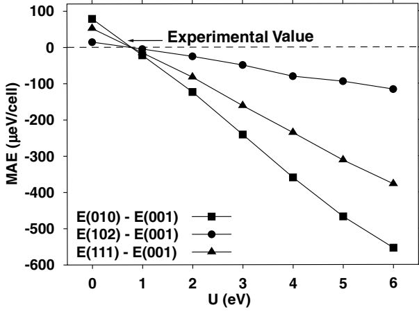
Fig. 3. The magneto-crystalline anisotropy energies MAE for \text{CrO}_2 as functions of U . The experimental value of MAE E[010] - E[001] = 15.6 \mu\text{eV} per cell is shown by arrow.
